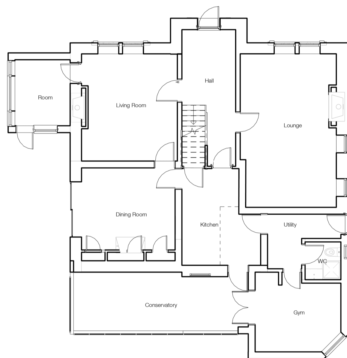
Existing GA Plan - Level 00
