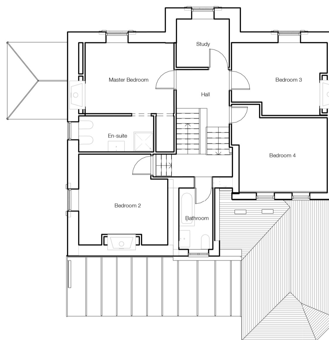
Existing GA Plan - Level 01
