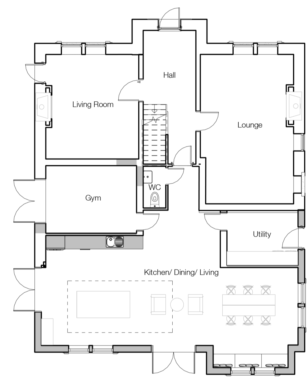
Proposed GA Plan - Level 00 1 : 100
