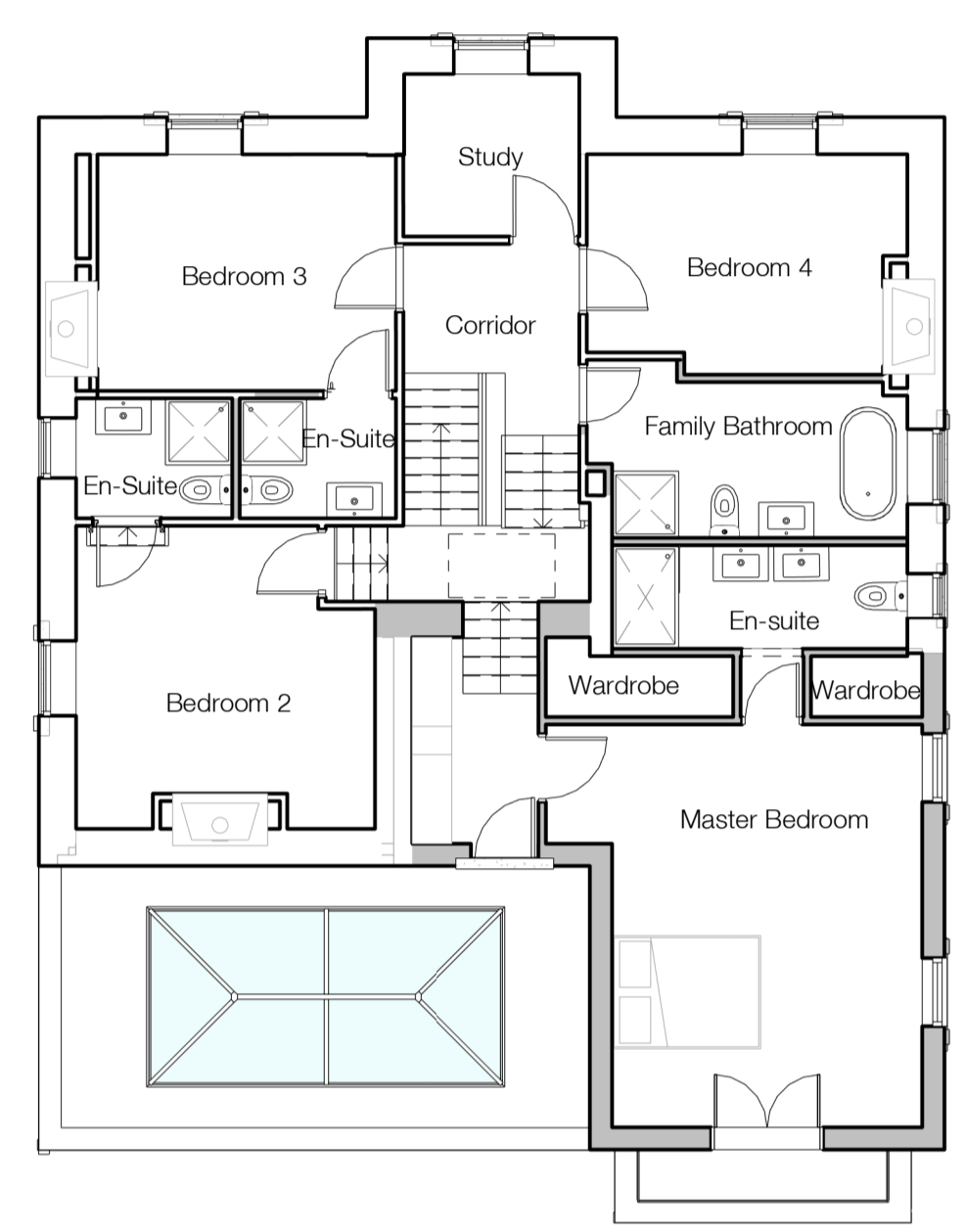
Proposed GA Plan - Level 01 1 : 100
