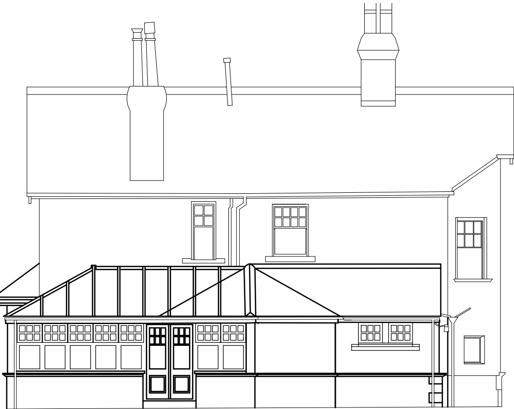
North West Elevation - Existing - 1:100
